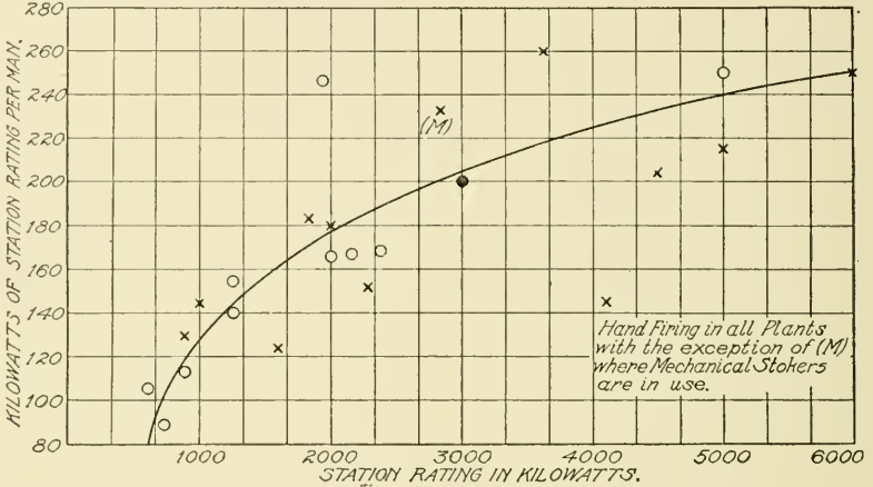
Fig. 164. Curve Showing Relation of Man Labor to Kws. Produced
